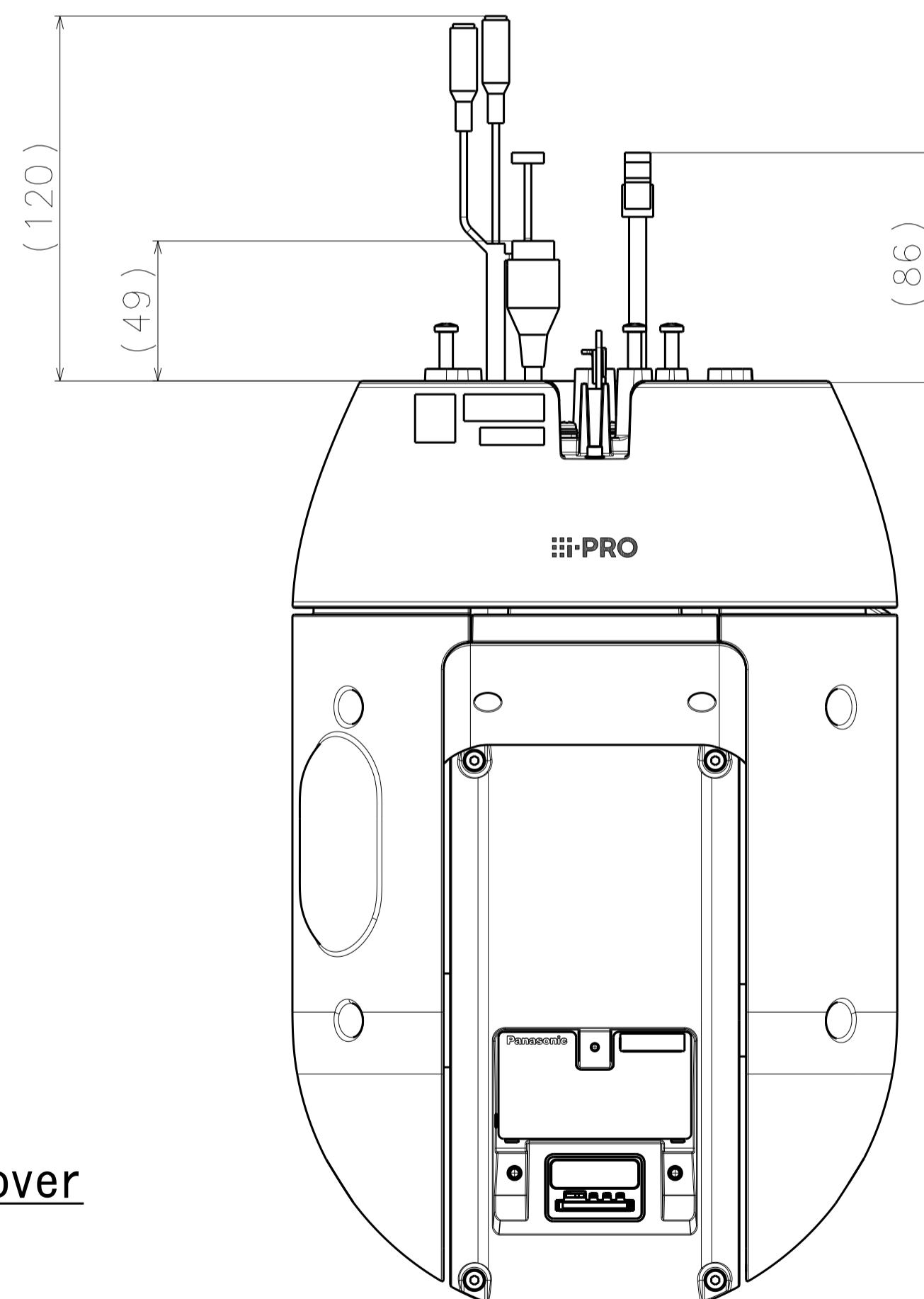
Remove SD slot cover / Cable cover
