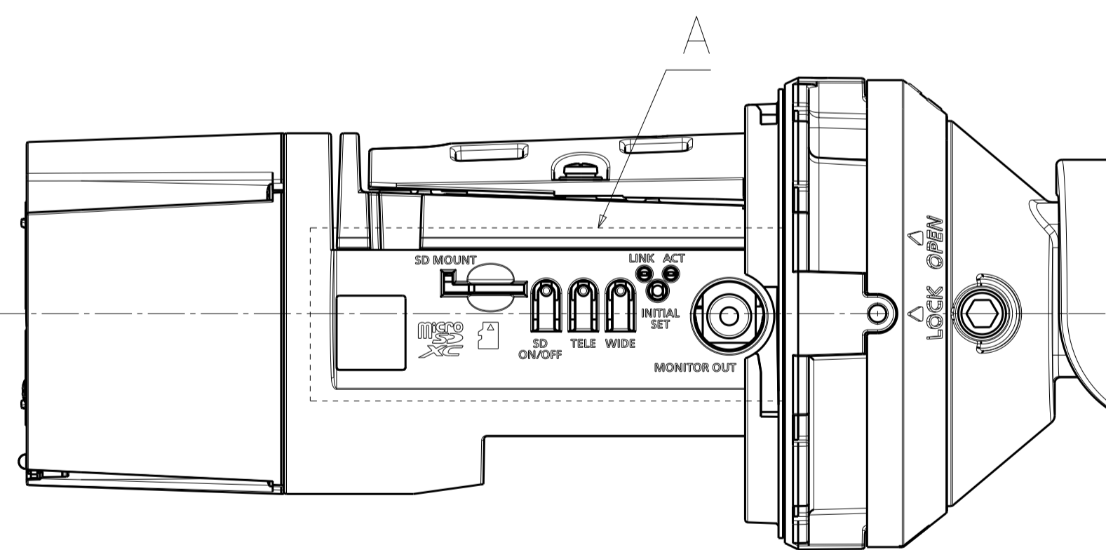
Detail A (2:1)
